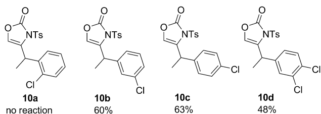
Scheme 7. Trends observed in the oxidative Heck arylation of cyclic enamides with chloro-substituted aryl boroxines.
